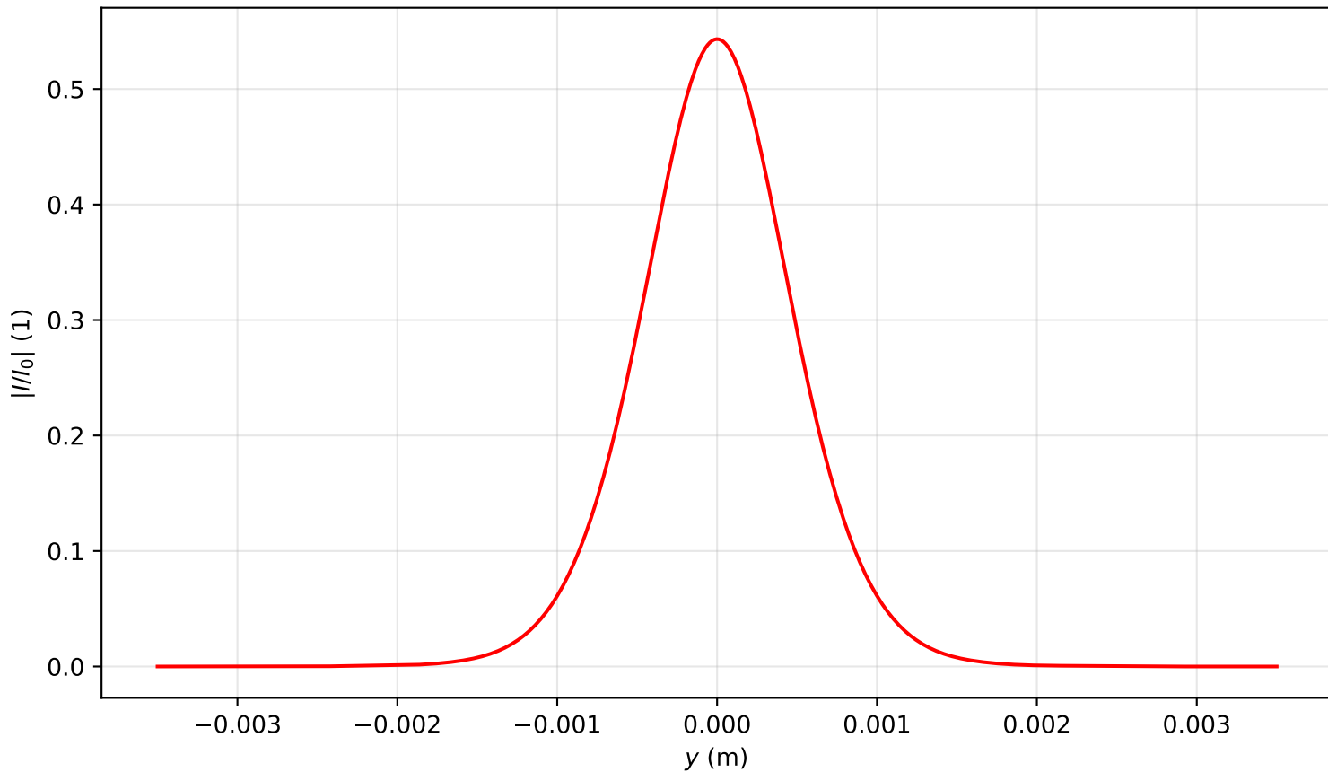
Intensity profile I(x=0, y, z=3.105)/I_0 , P_{in}=0.5P_{cr} , artificial time
